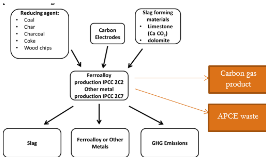
Figure 11: Ferroalloy production process pathway
