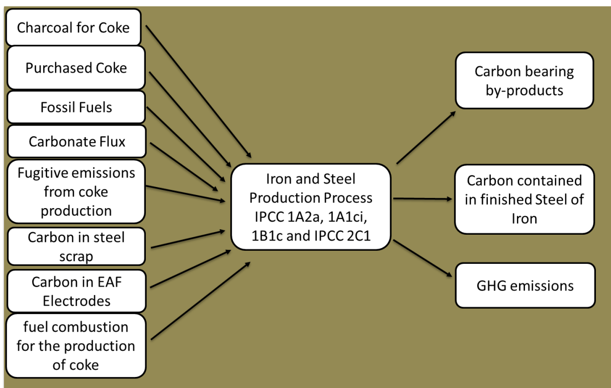
Figure 22.1 Process emissions flow for iron and steel (Including IPCC codes 1A2a, 2C1, 1A1ci and 1B1c)
