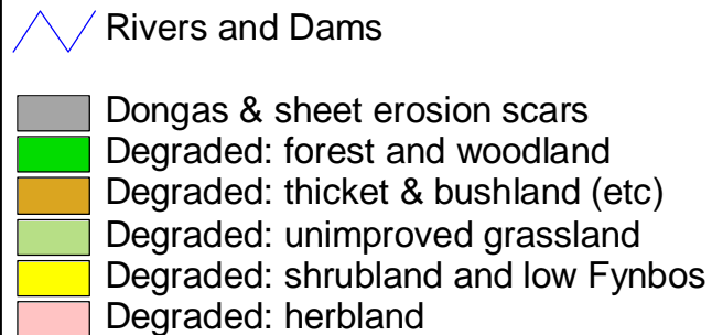
Degraded Class - Land-cover Map for the Berg Catchment
