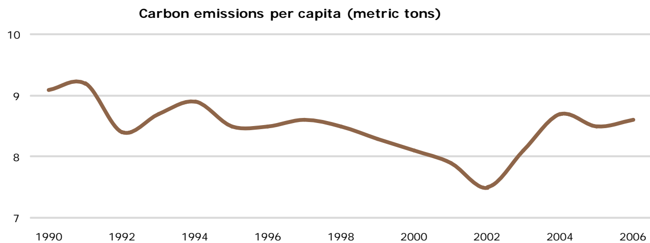
Figure 48: Total carbon emissions per capita in metric tons
