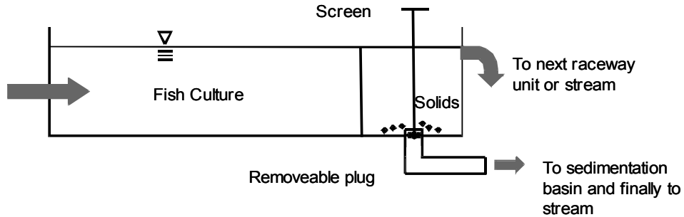
Figure 8. Illustration of the use of the end of a raceway for solids removal. Drawing is not to scale.
