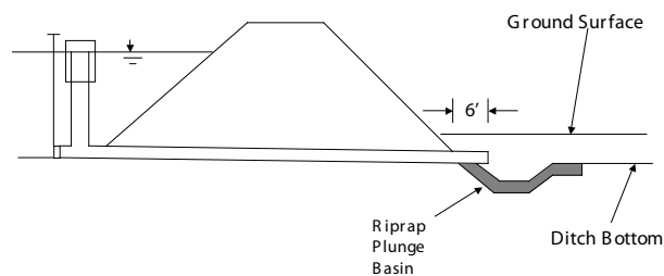
Figure 3. Cross-section of a pond embankment showing the drainage structure.
