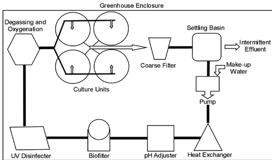
Figure 6. Illustration of an indoor, intensive aquaculture system with waste treatment processes. Drawing is not to scale.
