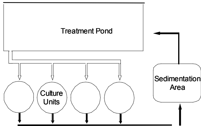
Figure 5. Illustration of aquaculture production systems with intensive culture units, sedimentation area, and treatment pond. Drawing is not to scale.
